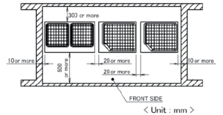
● The example of installation required space
